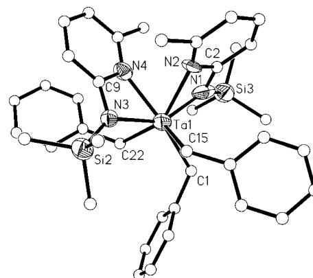
Figure 2. Molecular structure of 5 ; selected bond lengths [Å] and angles [°]: Ta–C1 2.250(11), Ta–N2 2.382(10), Ta–N4 2.248(10), Ta–N1 2.069(11), Ta–N3 2.212(9), Ta–C15 2.247(11), Ta–C22 2.318(10), N2–C2 1.379(16), N4–C9 1.355(14), N1–C2 1.375(15), N3–C9 1.391(13); C1–Ta–C15 81.09(5), C1–Ta–C22 76.15(4), C15–Ta–C22 130.18(5), N1–Ta–N2 60.31(4), N1–C2–N2 109.77(12), Ta–N1–C2 101.02(8), Ta–N2–C2 87.22(9), N4–Ta–N3 61.44(3), Ta–N3–C9 93.36(7), Ta–N4–C9 92.80(7), N4–C9–N3 112.12(11).
