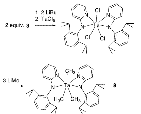
Scheme 6. Synthesis of 7 and 8 .
