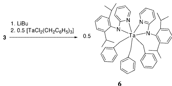
Scheme 5. Synthesis of 6 .
