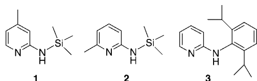
Scheme 3. Applied aminopyridines.
