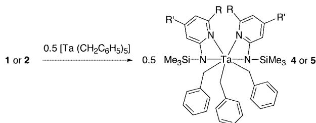
Scheme 4. Synthesis of 4 and 5 ( 4 : R = H, R' = CH 3 ; 5 : R = H, R' = CH 3 ).
