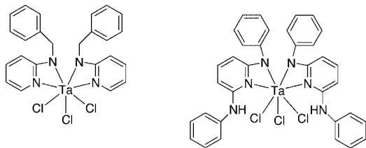
Scheme 7. Structures of 9 and 10 .
