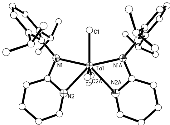
Figure 4. Molecular structure of 8 ; selected bond lengths [Å] and angles [°]: C1–Ta1 2.190(6), C2–Ta1 2.203(4), N1–Ta1 2.105(3), N2–Ta1 2.332(4), N1–Ta1–N1A 154.86(19), C1–Ta1–C2 106.89(12), N1–Ta1–C2 93.23(16), C2A–Ta1–C2 146.2(2), N1–Ta1–N2 145.88(13), N1–Ta1–N2 59.25(13), C1–Ta1–N2 136.67(9), C2–Ta1–N2 77.25(16), N2–Ta1–N2A 86.65(18).
